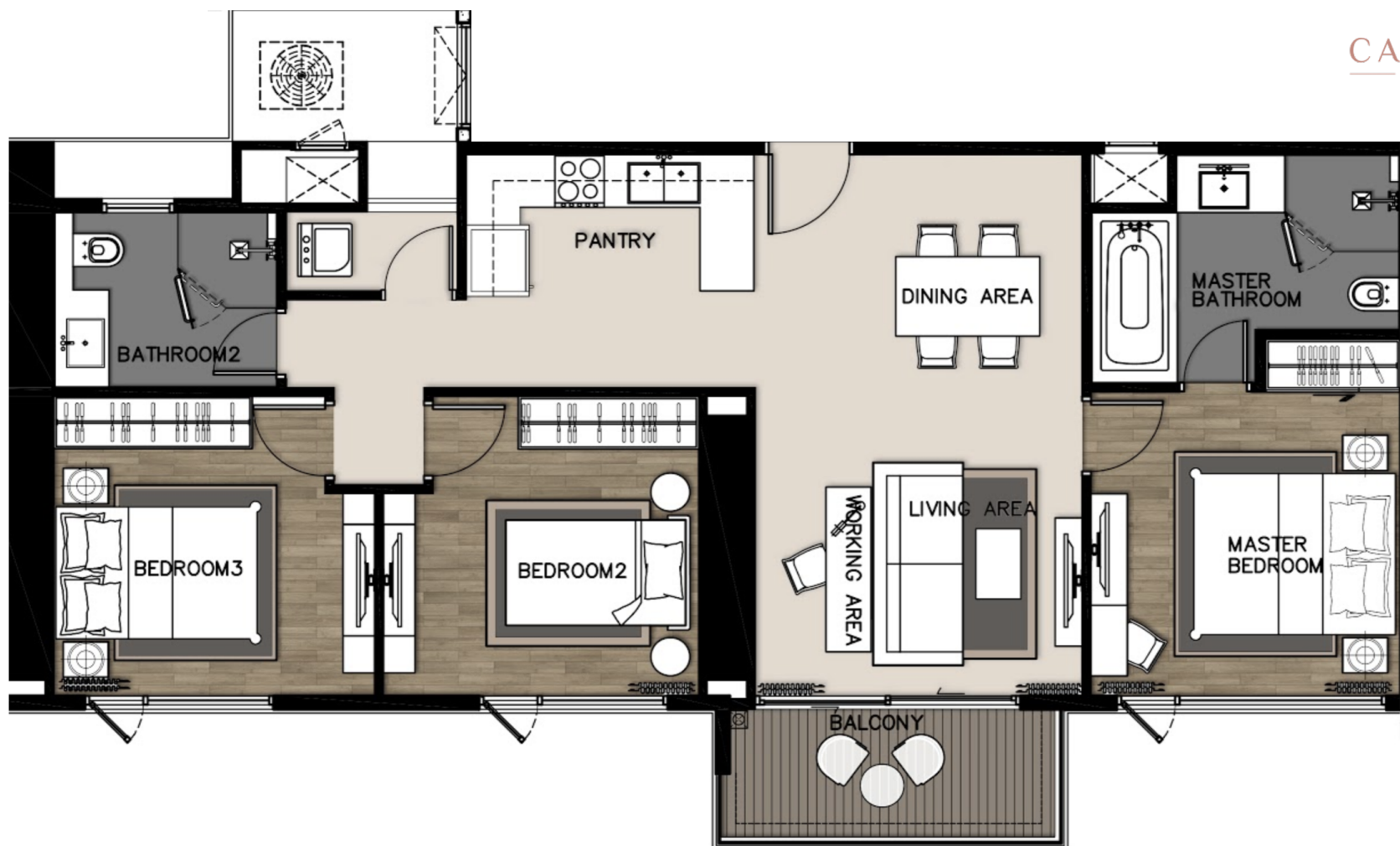
Unit Layout C3 3 Bedroom 3 Bathroom 93 SQM
